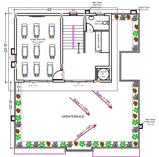
TERRACE FLOOR PLAN 792.66 SFT
