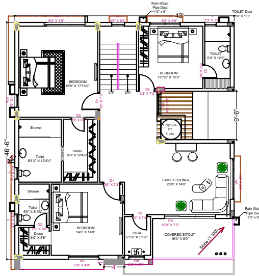
FIRST FLOOR PLAN 1950.81SFT
